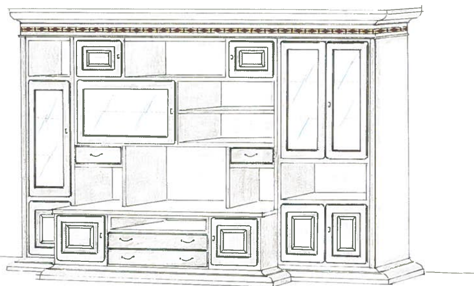
Art. CL865/Z | 330 x p 42/54 x h 240 - W 130 D 16 1/2 - 21 2/8 H 94 1/2
