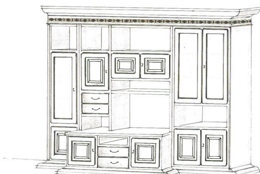
Art. CL865/O | 300 x p 42/54 x h 240 - W 118 1/8 D 16 1/2 - 21 2/8 H 94 1/2
